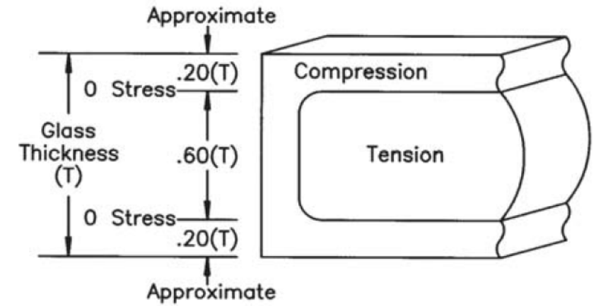
Heat-Treated Glass Compression and Tension Zones
