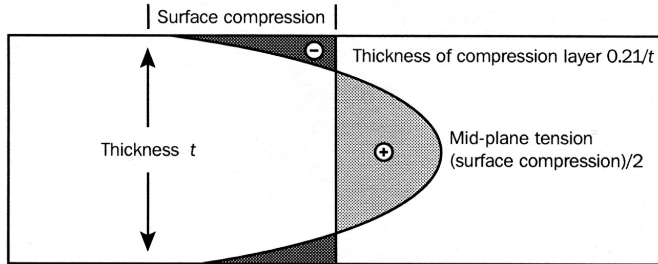
Stress distribution through thickness
