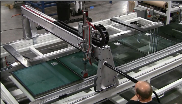
Semi-Automated Structural Glazer
