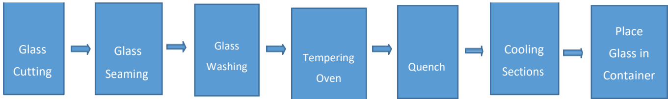
Figure 1: Tempering Process
