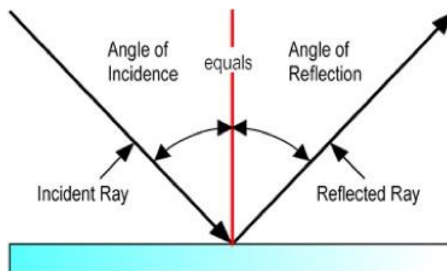
Figure 1: Reflection law
