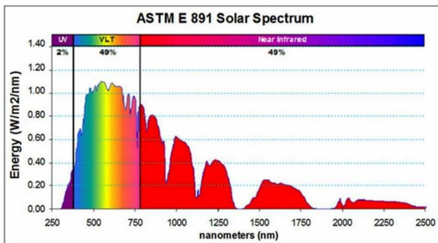
Figure 2: Solar Spectrum
